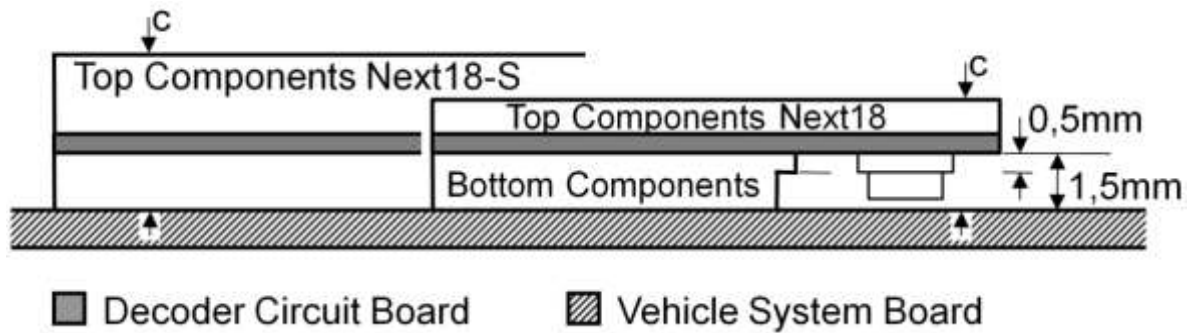
Figure 4: Decoder side view
